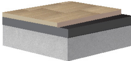
AttainSilence 2.5.5 2.5mm (0.10") Attain over 5.0mm (0.20") ECOsilence
