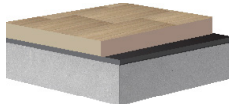
AttainSilence 4.2.1 4.2mm (0.17") Attain over 1.0mm (0.04") ECOsilence
